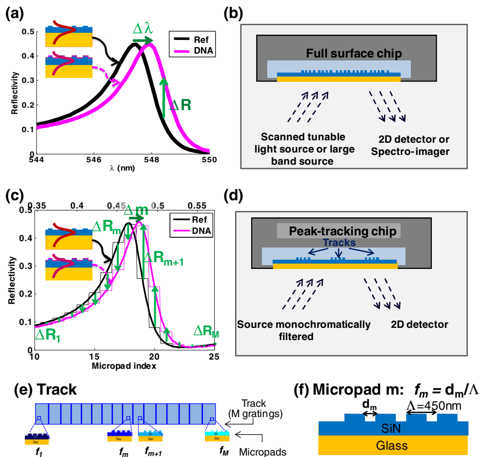
Fig. 1 a Typical shape of a resonant grating reflectivity spectrum, without ( black line , Ref) and with ( pink line , DNA) biological layer. Biological layer induces a shift \Delta\lambda of the reflectivity curve b Scheme of the optical set-up to measure spectral information in 2D: either a tunable light source with a normal camera, or a broad band source with spectro-imager detector are used c Implementation of SORCI: a nanopattern made of m=1\dots M grating micropads with varying geometry is used to scan around the resonance. Here m=10 to 25 covers the peak d Direct imaging set-up with our specially designed “Peak-tracking chip” e Detail of a track of M micropads with variable filling factor f . Grating in a micropad with period \Lambda=450 nm and groove width d_m . The air filling factor f_m varies from f_1=0.44 to f_M=0.57 in (e)
